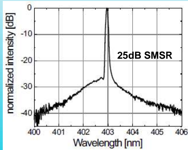
OSA Spectrum (Typical)
